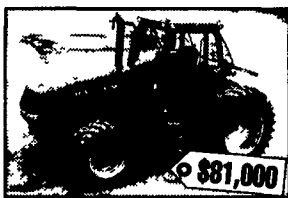
A 23804 2000 CIH MX 220 MFD Cab, 1334 Hours, 1000 Pto, 3 Pt Hitch, 3 Remotes, Powershift, Tires Fr-16.9 x 38, Rear-20.8 x 38, 185 HP
