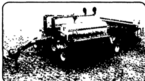
A 23337 Krause 5430 30' Drill, Demo Unit, High Residue Double Disc Parallel Link Openers, 3x13 Press Wheels, Hydraulic Fold
