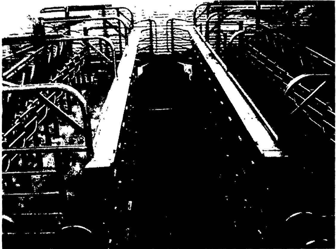
Blue Diamond Double 12 Stainless Steel Parallel Parlor
