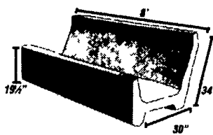
Slant-back J-style Feed Bunker
