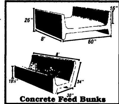
Concrete Feed Bunks
