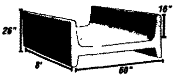
High Capacity H-style Feed Bunker
