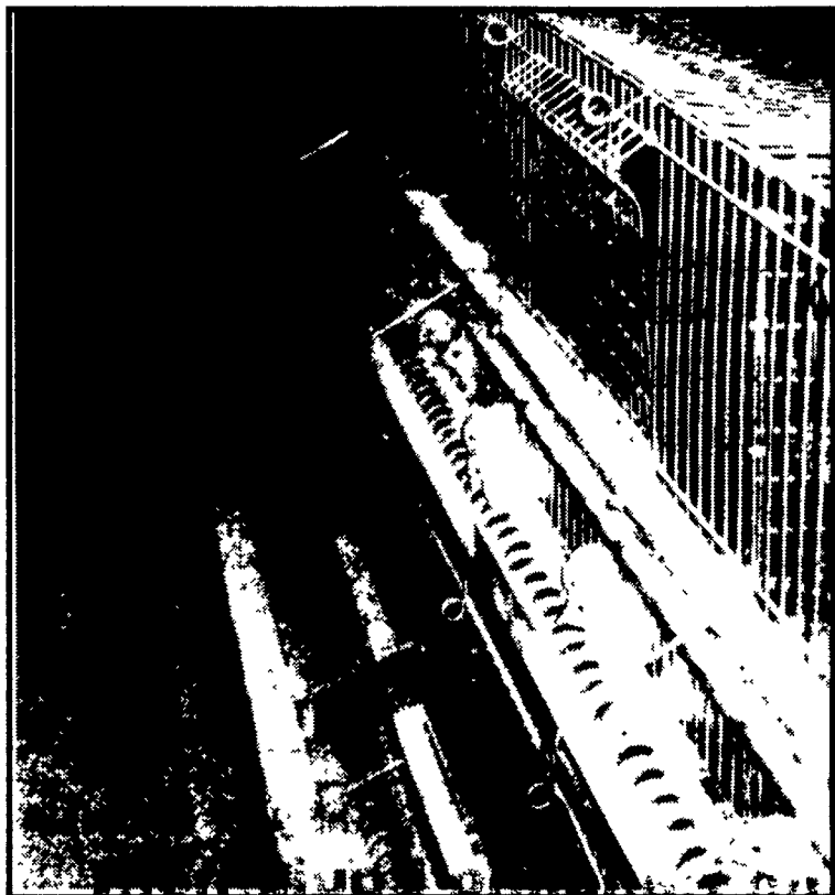
New Pullet house featuring Chore-Time cages with Ultraflo® feeder installed outside cage to save birds and reduce labor. Because the feeder is outside the cage, no manure is mixed with the feed as it is in other systems.
