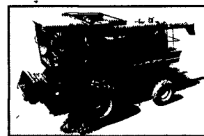
A 22724 1989 CIH 1680 2WD, 2654 Hours, Field Tracker, Specialty Rotor, GLM, Rock Trap, Tires Dr - 30 5 x 32, Steering - 14 9 x 24 SALE PRICE $48,500
