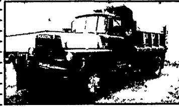
(1) 1979 MACK RD , Mack 200HP, 13 Spd, Spring Suspension, 11x20 Tires, Spoke Wheels, Single Axle, Green, Stk #P1488 $7,500
