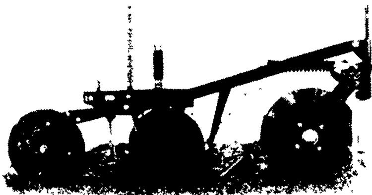
The proven Great Plains no-till system utilizes a coulters to prepare a mini-conventional seedbed for the openers to place the seed ... at the precise depth selected.
