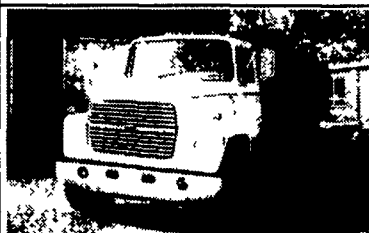
'86 FORD LN8000 16' Flat Dump, 3208 Cat, 210 HP, 5 Spd Trans., 2 Spd Rear, 33,000 GVW, Air Brakes $19,500
