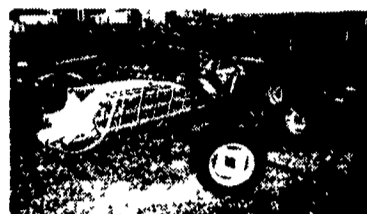
NH 256 Rake w/Dolly Wheel
