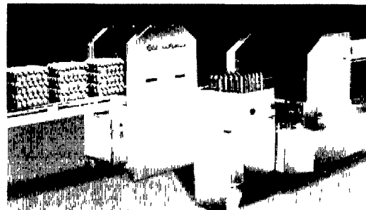
Diamond Systems 100 case per hour Farmpacker with tray stacker.
