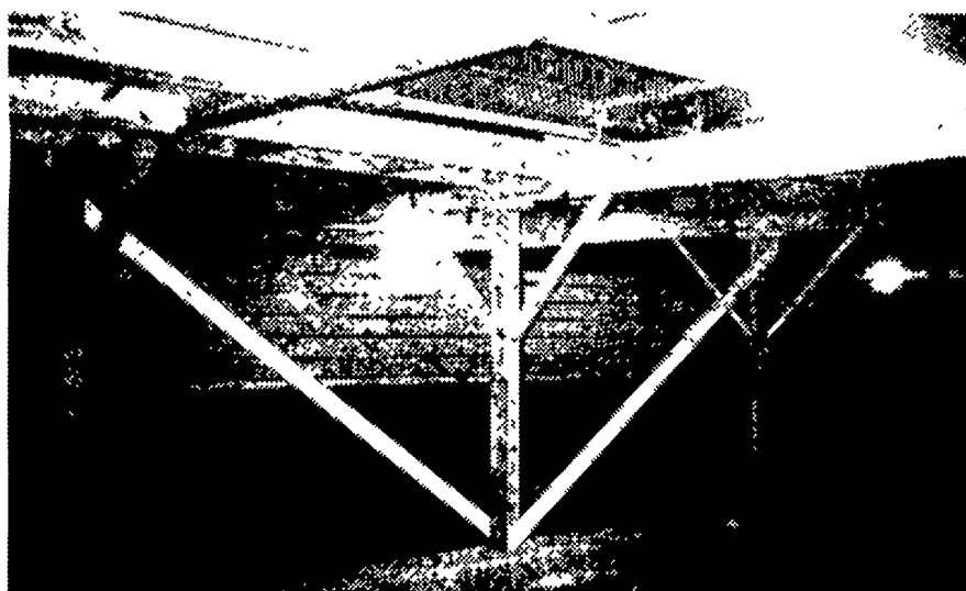
Dirt floor pit with concrete curbs, laminated engineered beams, painted steel from poured concrete wall and across ceiling.
