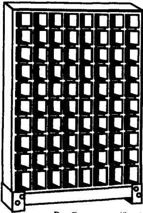
Bin Openings: 4" x 4 1/2" Bin Dimensions: 54" H x 35" W x 12" D
