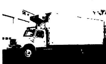
(1) 1990 INTERNATIONAL 4900 REEFER TRUCK IHC DT-466 210 H P Fuller 6 Speed Eaton Rears A/C P/S AM/FM Stereo, Dual 50 Gal Tanks, Hackney 24' Reefer Body, C/S Side Door Rear Roll Up Door
