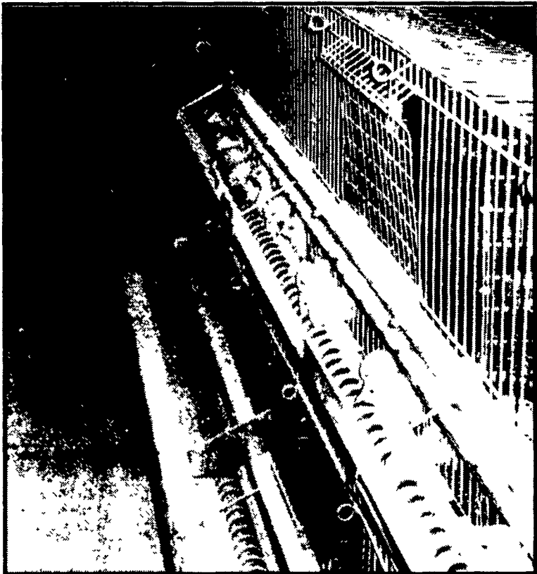
New Pullet house featuring Chore-Time cages with Ultraflo® feeder installed outside cage to save birds and reduce labor.
