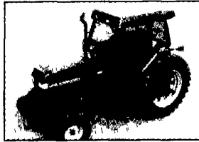
B 21477 CIH 5240 2WD Tractor, 1992, 1824 Hours, 10x16 & 18 4x38 Tires, 2 HYD Valves, 540/1000 PTO, 3 pt. Hitch
