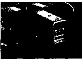
A 16089 MF 245 Tractor, 5017 Hours, 9 5LX15 & 13 6X28 Tires,
