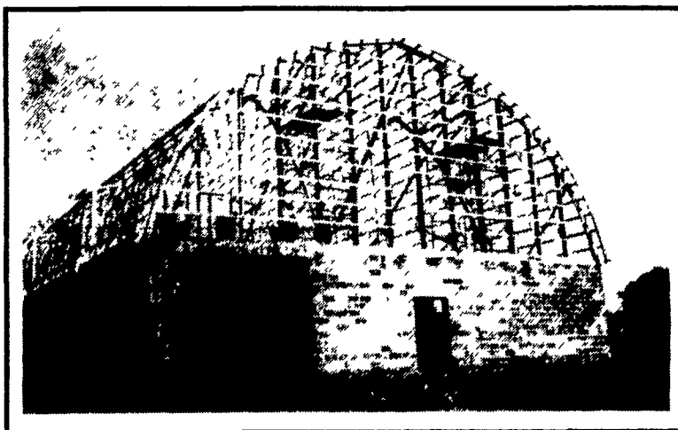
Gothic Arches To Match An Existing Building
