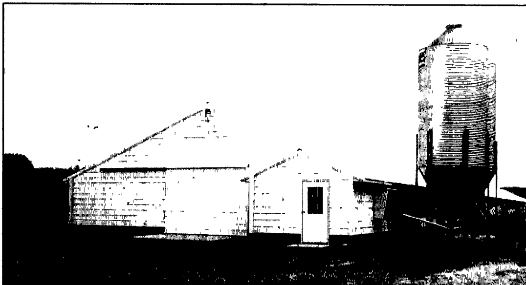
All new solid wall tunnel ventilated broiler house constructed by Northeast Agri Systems. Walls are 2x6 pole construction.
