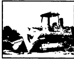
Dresser Crawler with 4 In 1 Loader, 160 HP Cummins.
