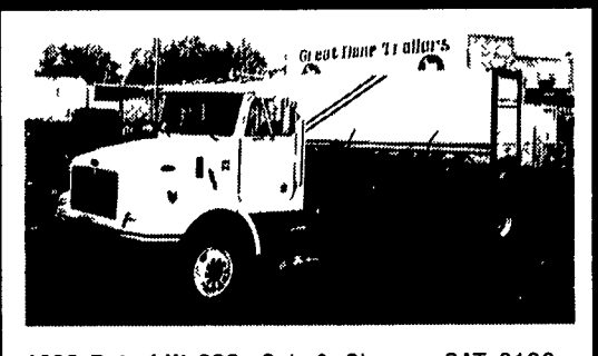
1998 Peterbilt 330, Cab & Chassis CAT 3126 - 250 HP, 12,000 FA, 21,000 RA, 33,000 GVW, 6-spd. Trans, for 24 Ft Body
