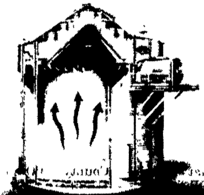
Outside air from the cooling fan captures heat from the hot dried grain, and rises through the new layer of wet grain above
