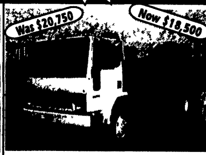
1993 Ford Cargo CF8000, Cab & Chassis Only, 7.8L 210 HP Engine, 6-Speed, 12,000 Front Axle, 21,000 Rear Axle, 225" WB, 195 CA, 33,000 GVW, Air Brakes, Low Miles LIKE NEW
