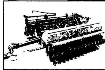
GP 30' Drill, Solid Stand Conventional, Folding 4x12 PW, 12-12 1/4" Disc (20439)
