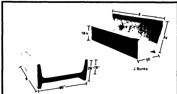
Concrete Feed Bunks
