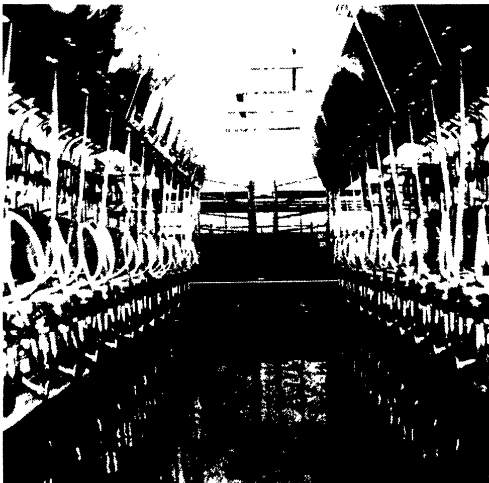
300 Cow, 6 Row Laminated Rafter Free Stall Barn With Concrete Slatted Manure Pit.
