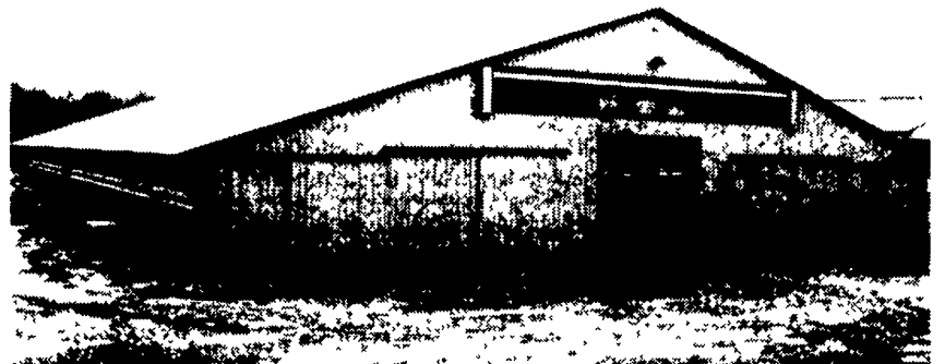
300 Cow, 6 Row Laminated Rafter Free Stall Barn With Concrete Slatted Manure Pit.
