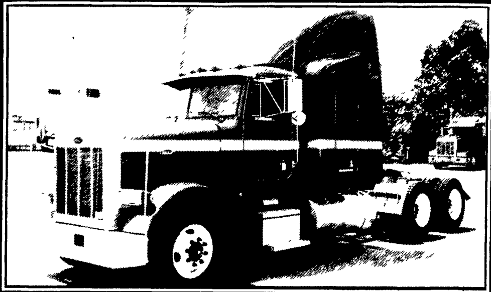
1991 PETERBILT 378-119 JAKE 3406B-350 ENG., RTO 14609B TRANS., DS402-4.11 R. AXLE, AIR LEAF SUSPENSION
