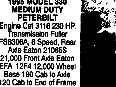
1995 MODEL 330 MEDIUM DUTY PETERBILT Engine Cat 3116 230 HP, Transmission Fuller FS6306A, 6 Speed, Rear Axle Eaton 21065S 21,000 Front Axle Eaton EFA 12F4 12,000 Wheel Base 190 Cab to Axle 120 Cab to End of Frame 195 33,000 GVW
