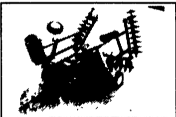
Kr. 1924 Rockflex Disc, 21' Cut Width, New 22" Blades, 9" Spacing, New Paint (8766)
