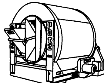
Tumble mixers
