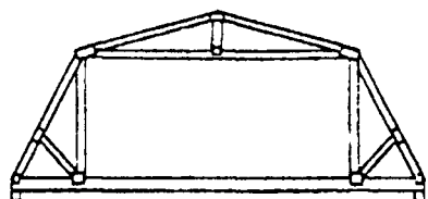
GAMBREL ATTIC
