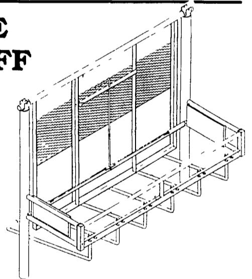
All Gates & Fencing Made Of 1.9" Outside Diameter High Yield Steel Tubing With 13 Ga. Wall
