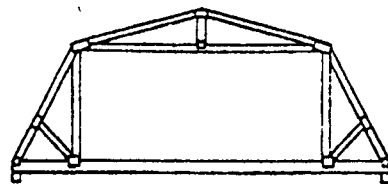
GAMBREL ATTIC
