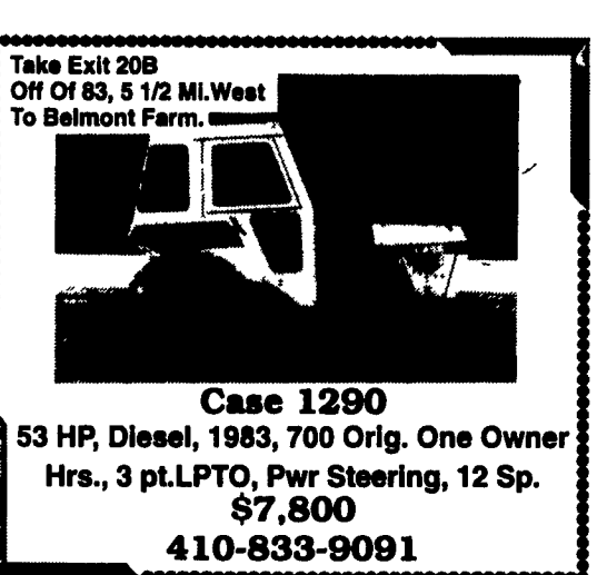
8830 Case IH 14 Ft. Windrower; 875 Hrs; w/Hyd. Tilt and Hyd. Header Float; 21.5L x 16.1 Turf Tires $27,500 717-263-8091
