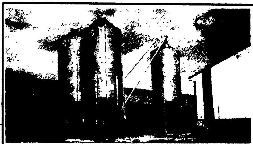
Two CHORE-TIME Next Generation 25.6 ton storage bins with transfer auger to Chore-Time weigh bin. Chore-Time feed screener and dual Model 90 filter system.
