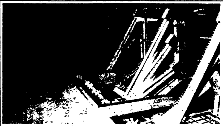
CHORE-TIME ® Variable speed rubber finger egg collectors. CHORE-TIME ® 4 tier 24"x20" Duracage, 9 birds per cage with push in doors.
