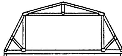
GAMBREL ATTIC
