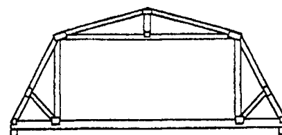
GAMBREL-IN-ATTIC
