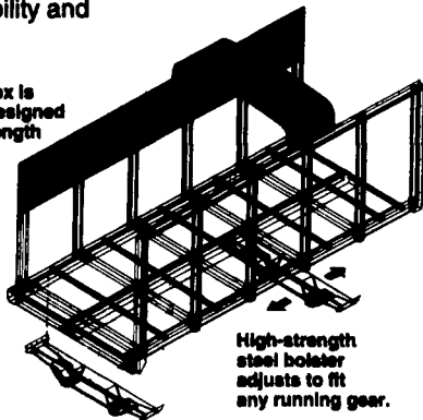
Optional Miller Pro Running Gear • Choice of models from 10 - 14 tons • Automotive-type steering • C-Channel design for best stability and tracking
