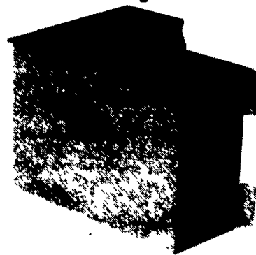
2AC Multi-Purpose Fountain Waters calves, sheep and goats. Perfect for box stalls, small lots or fencelines Waters up to 40 cattle/100 calves Part No. 12295 10" x 24" x 18" high Electric (286W, CSA approved)
