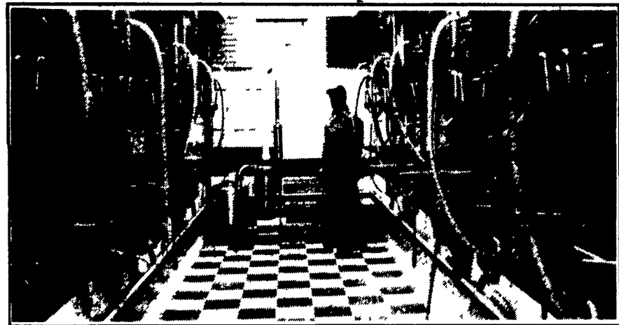
All New Alfa-Laval Agri Double 6 Herringbone Parlor With Blue Diamond Suspended Indexing Stalls Complete With Plate Cooler, Take-Offs & Milk Meters.
