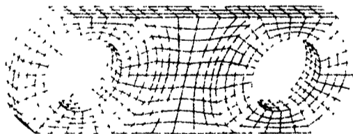
The full round bushing distributes force in a symmetrical pattern to the sidebar.
