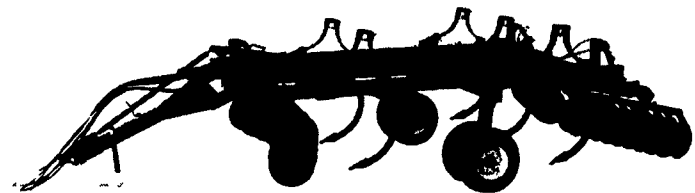
Landcommander 3 shank - 30" spacing, disc spacing: 15" front - 7 1/2" rear 5 shank - 24" spacing, disc spacing: 15" front - 7 1/2" rear
