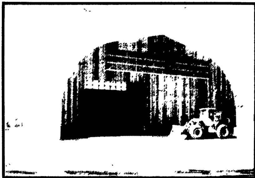
80'x80' Salt Storage - Ceiling Is High Enough To Raise Dump Trk. Bed
