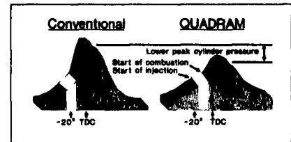
Lower peak cylinder pressures and stresses result when less combustion takes place prior to TDC.
