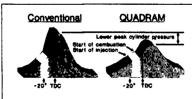
Lower peak cylinder pressures and stresses result when less combustion takes place prior to TDC.
