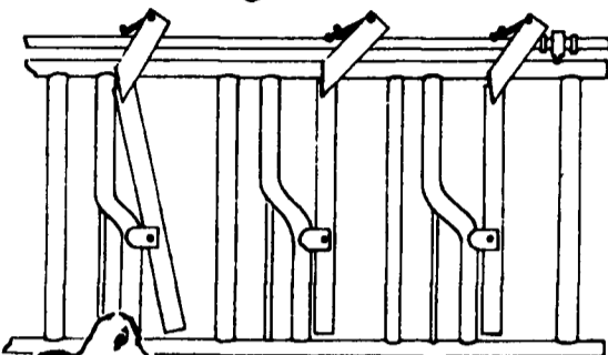
Automatic Headlock
