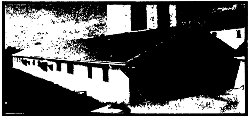
Dairy barn exterior featuring: clear span trusses, plain aluminum strong rib roof and painted aluminum strong rib gable walls.
