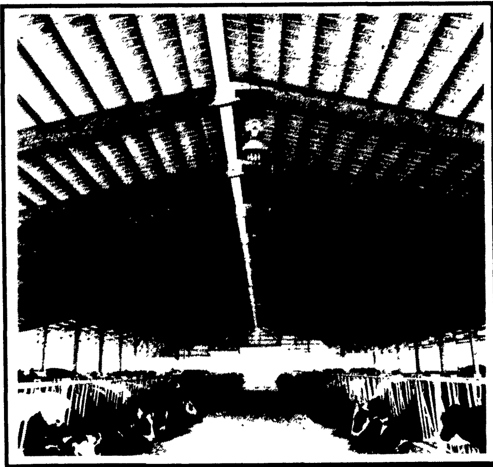
108' x 204' (Interior view) Free Stall Barn Featuring Glu-lam straight beams & Glu-lam posts
